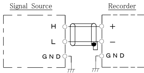
Fig. 5.1 Connection of Signal Lines (an ordinary method of signal line connection)
