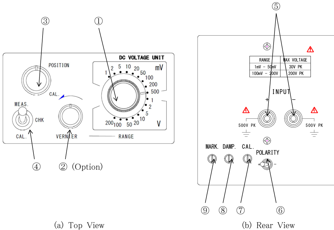
Fig. 4.4 Amplifier Unit
