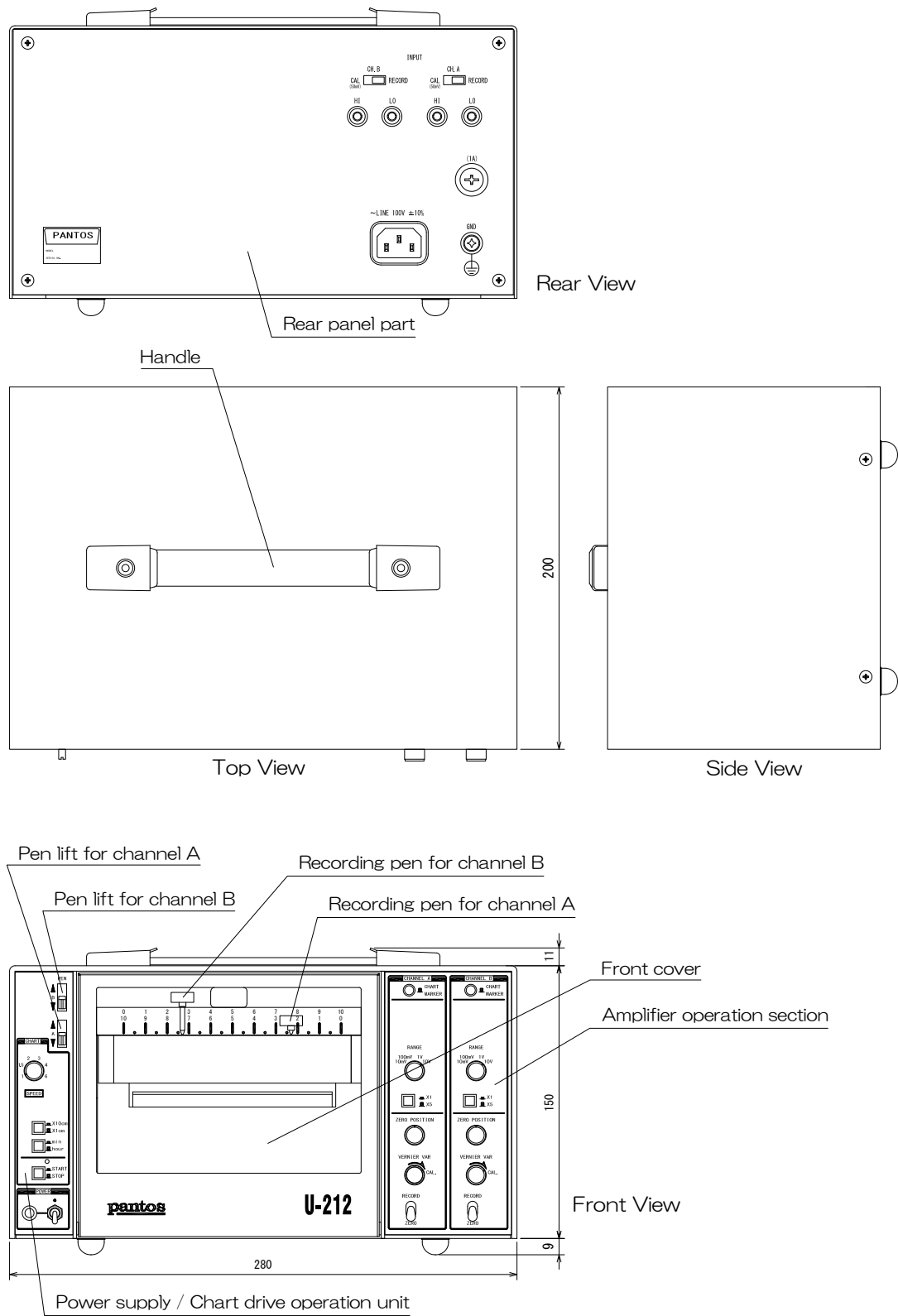
Fig.4.1.1 External drawing
